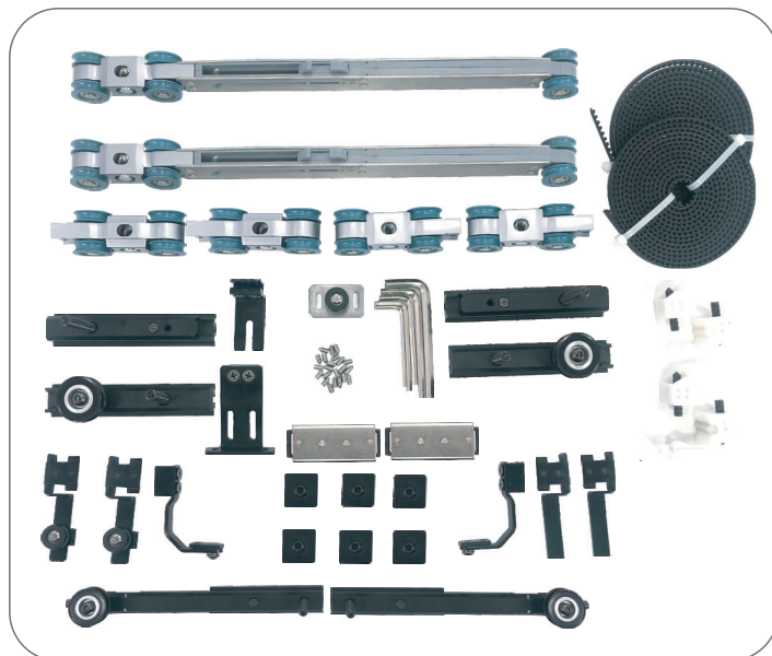
Telescopic Sliding Set - 1 Fix 3 Sliding Door
