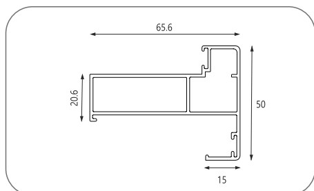
Outer Frame Profile
