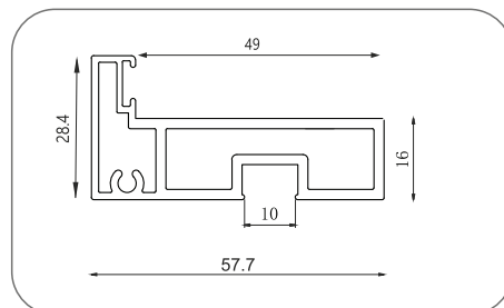
Slim Outer Frame Profile
